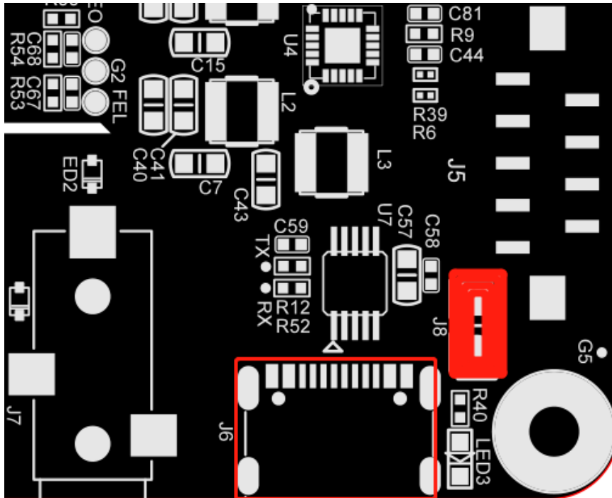
USB-C 5V IN
